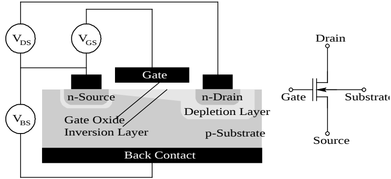
Fig.1 Crosssection and circuit symbol of an n-type metal-oxide-semiconductor field-effect transistor
