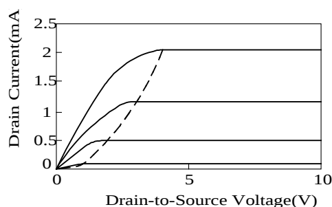
Fig.3 I-V characteristics of an n-type MOSFET with V_G = 5V (top curve), 4V , 3V and 2V (bottom curve)
