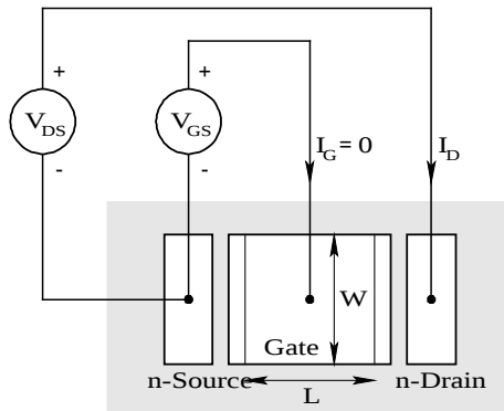
Fig.2 Top view of an n-type metal-oxide-semiconductor field-effect transistor (MOSFET)
