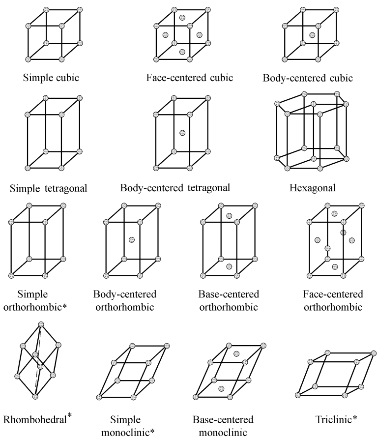
Figure 1.14 The fourteen types of Bravais lattices grouped in seven crystal systems
