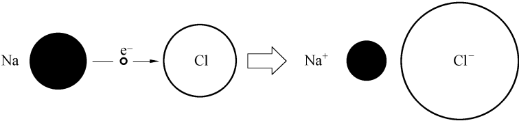
Figure 员圆 Ionic bonding
