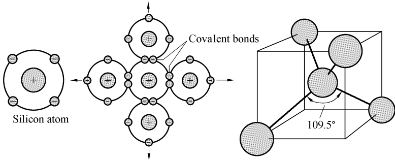
Figure 员猿 Covalent bonding
