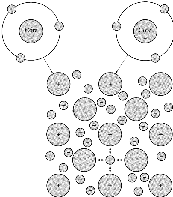
Figure 1.10 Metallic bonding
