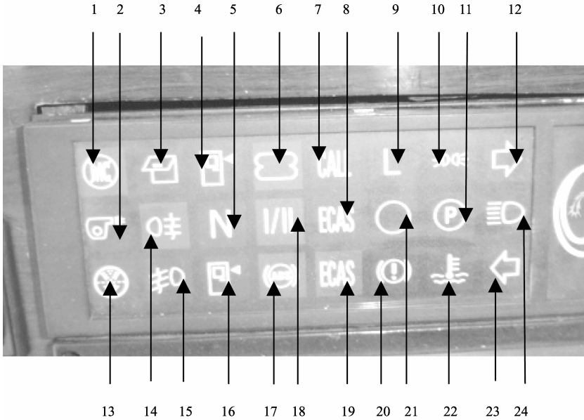
图 1-7 监视屏
