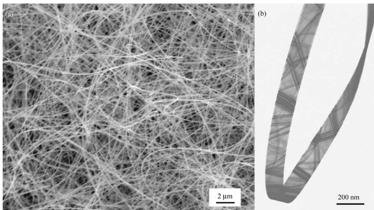
Fig 3 Ultra-long nanobelt structure of ZnO (a) SEM image of the as-synthesized ZnO nanobelts with high purity and crystallinity; (b) Bright-field TEM image showing the bent belt shape . The contrast observed in TEM image is due to bending strain .
