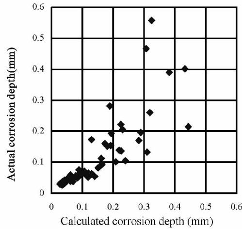
Fig. 11 Comparison of the calculated and the actual corrosion depths of 17 steels after 1-, 2-, 4-, 8-, 16-year exposure at Wanning, China
