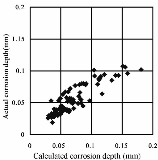
Fig. 10 Comparison of the calculated and the actual corrosion depths of 17 steels after 1-, 2-, 4-, 8-, 16-year exposure at Beijing, China
