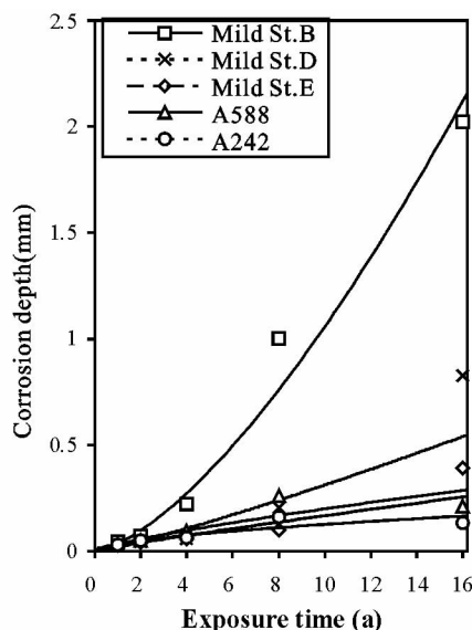
Fig. 4 Atmospheric corrosion of 5 different steels after 16-year exposure at Wanning, China (the symbols indicate the actual data, and the lines are the regression curves)
