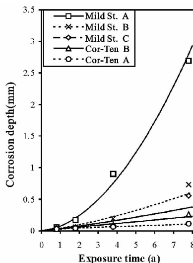
Fig. 2 Atmospheric corrosion of various steels at Wanning, China (the symbols indicate the actual data, and the lines are the power function regression curves)
