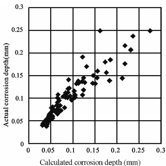
Fig. 8 Comparison of the calculated and the actual corrosion depths of 17 steels after 1-, 2-, 4-, 8-, 16-year exposure at Guangzhou, China
