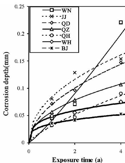
Fig. 1 Atmospheric corrosion of a mild steel at seven different exposure sites (the symbols indicate the actual data, and the lines are the power function regression curves)
