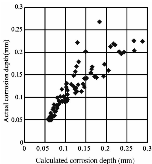
Fig. 7 Comparison of the calculated and the actual corrosion depths of 17 steels after 1-, 2-, 4-, 8-, 16-year exposure at Jiangjin, China
