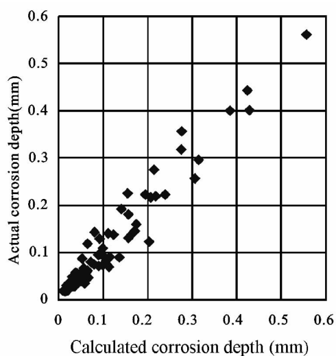
Fig. 9 Comparison of the calculated and the actual corrosion depths of 17 steels after 1-, 2-, 4-, 8-, 16-year exposure at Qionghai, China
