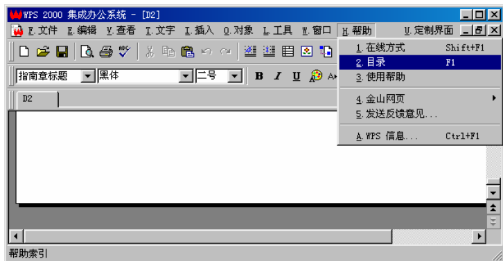
图1.2 帮助菜单
