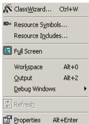
图 1.4 View 菜单
