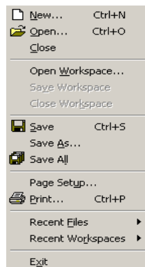
图 1.2 File 菜单
