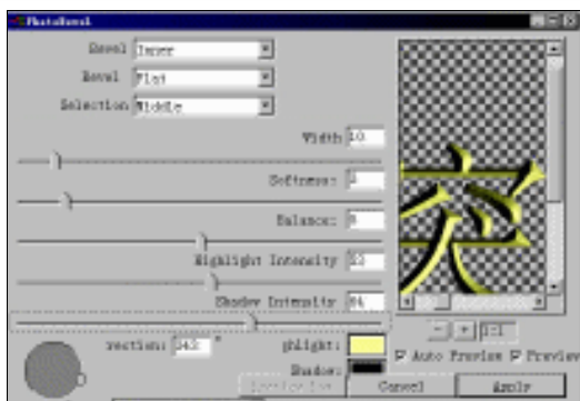
图 3-4 PhotoBevel 滤镜
