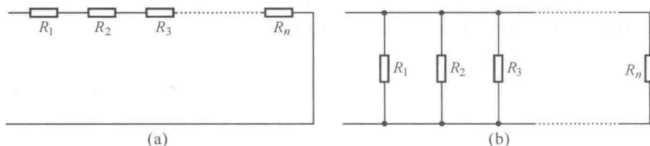
Figure 2.1 Resistance in serial and parallel circuits
