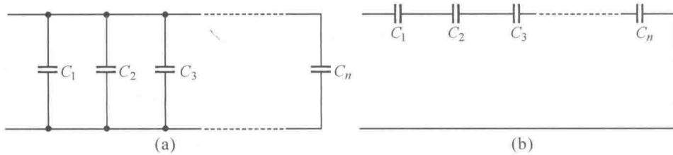
Figure 2.2 Capacitance in parallel and serial circuits
