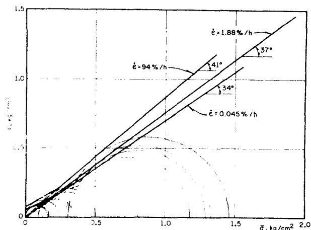
Fig. 6 Mohr envelopes. Effective stresses
