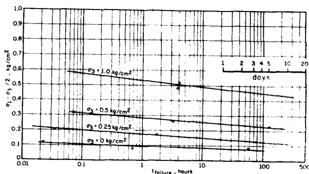
Fig. 7 Maximum deviator stress versus time to failure
