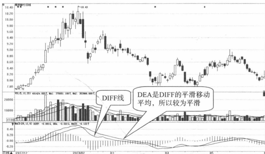
图 1-2 DIFF 线与 DEA 线
