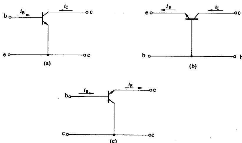
Fig. 1-4 Three Basic Ways of Connecting Transistors in A Circuit
