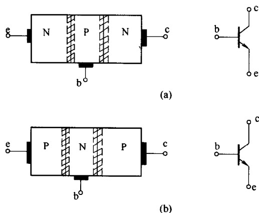
Fig. 1-3 P-N Junction and Transistor
