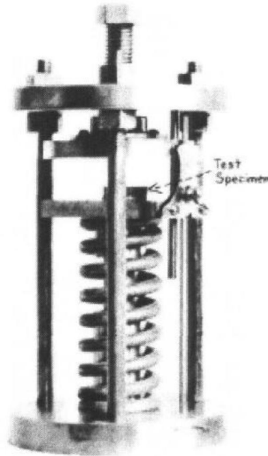
FIG. 1 Device for Compression Set Test, Using Calibrated Spring Loading, Test Method A
