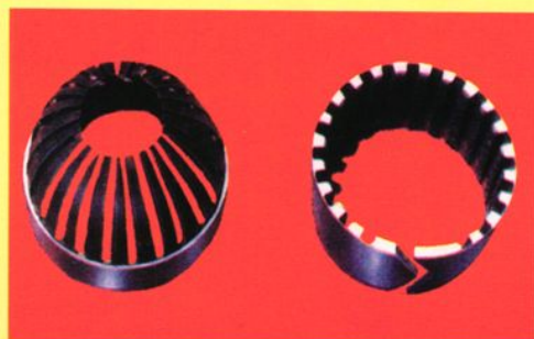
▼ 弹簧片和卡箍岩心爪
