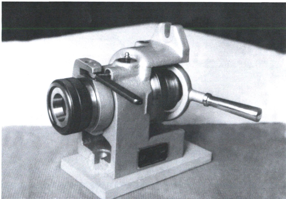
FNL100B型立卧等分分度头
