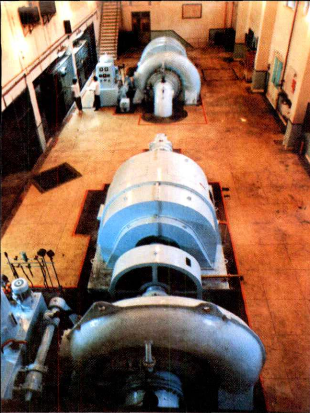
百丈漈二级站水轮发电机组
