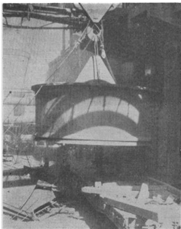
吊装高炉大钟及漏斗
