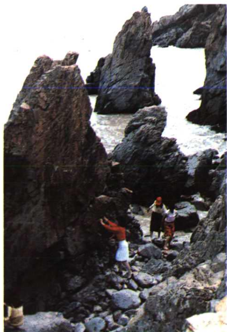
燕窝石笋
