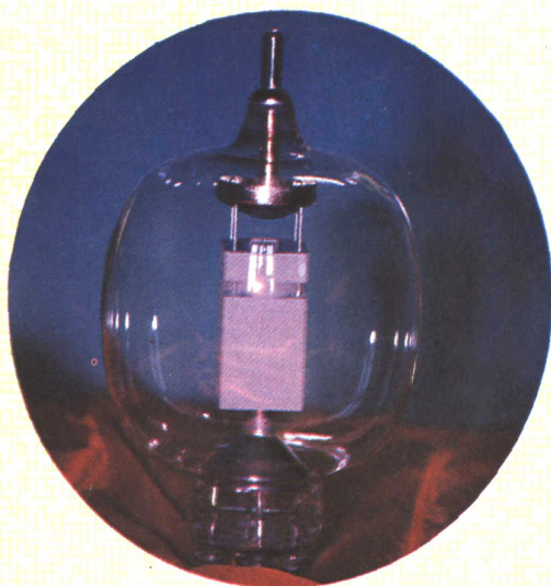
6T51 中功率發射管 6T51 medium power transmitting tube
