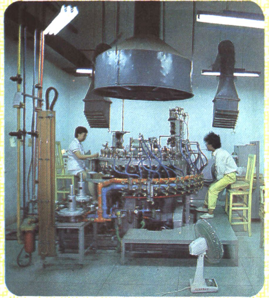
玻璃生產綫工人在製作玻璃零件 Workers on the glass tube production line are making glass tube envelopes.
