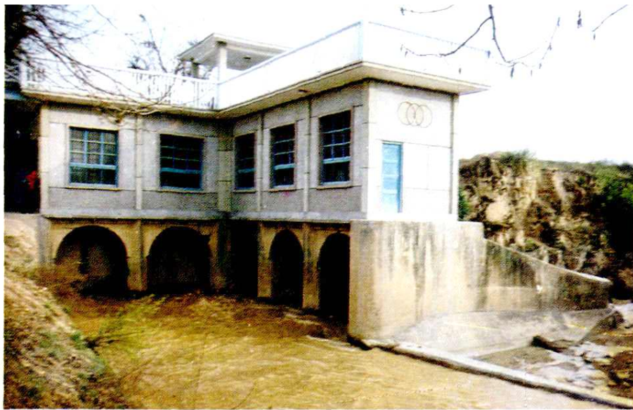
渠首进水闸
