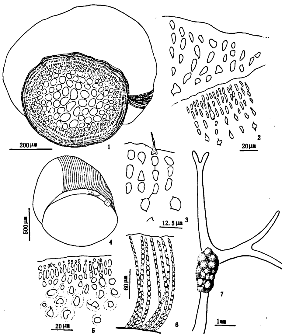
图2 莺歌海伊谷藻 Ahnfeltia yinggehaiensis Xia et Zhang 1. 藻体横切面 (AST 57—5799); 2. 轴的横切面, 示果胞 (AST 80—2331); 3. 果胞 (AST 80—2331); 4. 轴的横切面, 示辐射状的产孢丝 (AST 80—2331); 5. 精子囊横切面观 (AST 80—2331); 6. 产孢丝放大图 (AST 57—5799); 7. 果孢子体外形图 (AST 57—5799)。 Fig. 2 Ahnfeltia yinggehaiensis Xia et Zhang 1. Transection of frond (AST 57—5799); 2. Transection of frond, showing carpogonium (AST 80—2331); 3. Carpogonium (AST 80—2331); 4. Transection of frond, showing radiating gonimoblast filaments (AST 80—2331); 5. Transection of spermatangia (AST 80—2331); 6. Enlargement of gonimoblast (AST 57—5799); 7. Carposporophyte (AST 57—5799).
