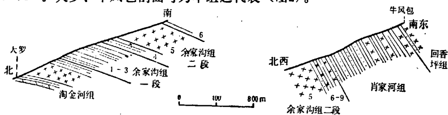
图 2 贵州印江大罗、牛风包余家沟组剖面略图 Fig. 2 Schematic sections of Yujiagou Formation at Daluo and Niufengbao, Yinjiang, Guizhou
