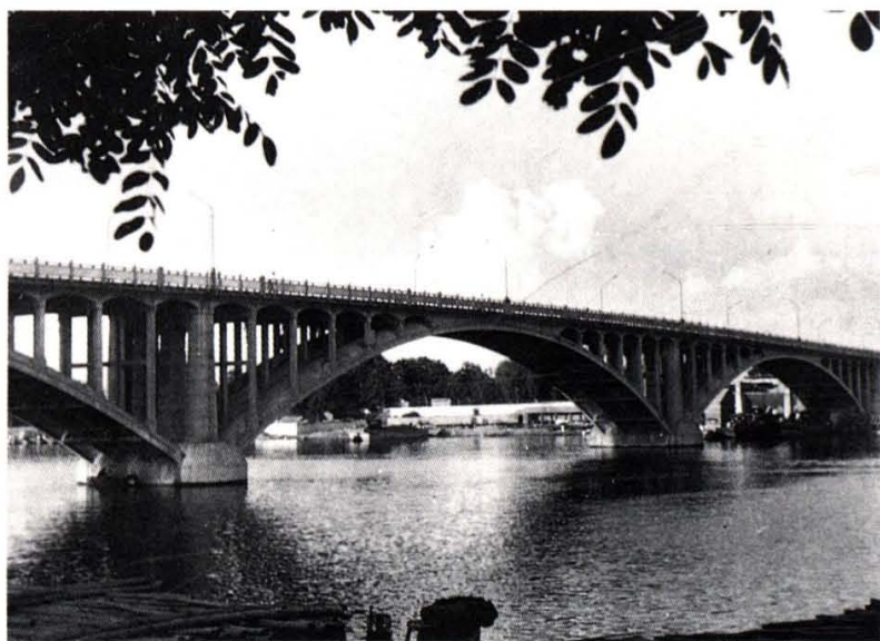
宿迁运河双曲拱桥
