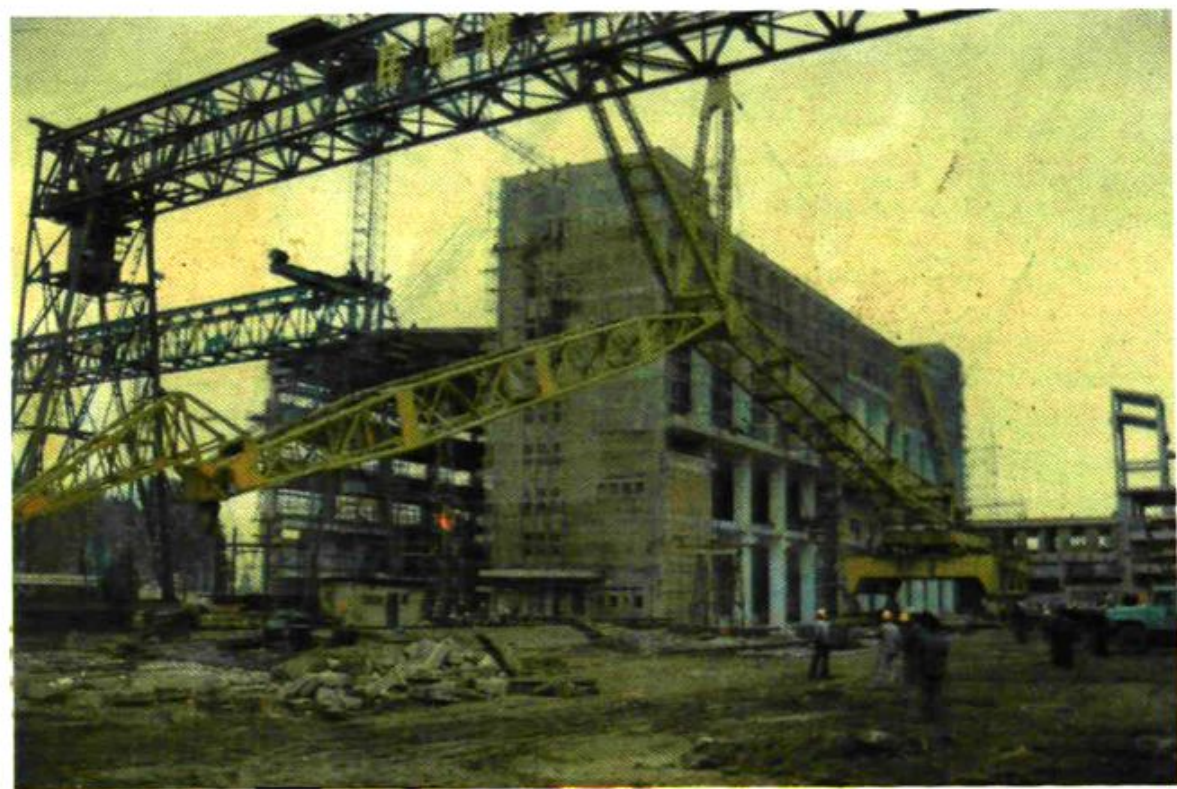
TQ-1300/70塔式吊车安装
