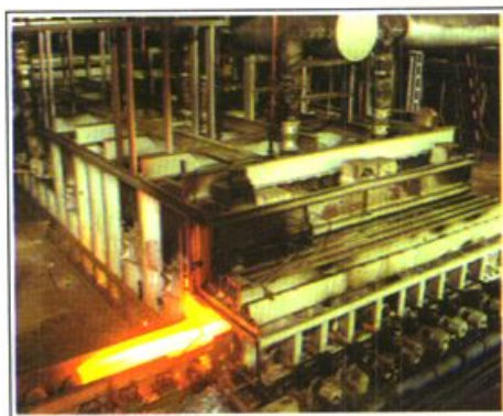
● 长钢步进式加热炉
