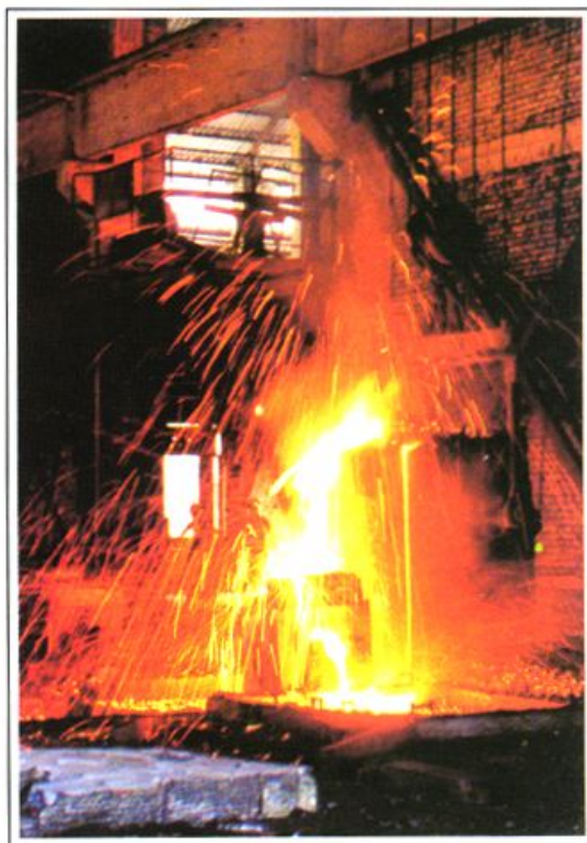
● 江油钛厂硅水出炉
