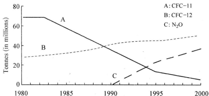
Three Damaging Gases to Ozone Layer
