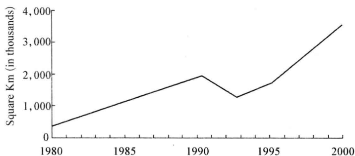
Ozone Hole Size over Antarctica
