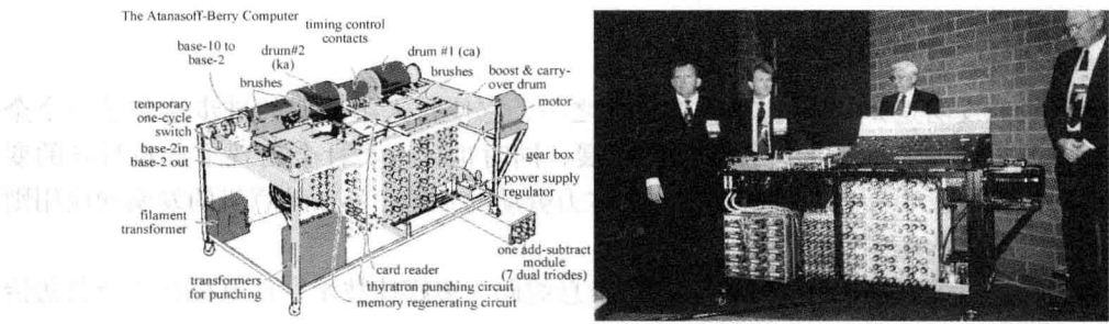
图 1-1 Atanasoff – Berry Computer
