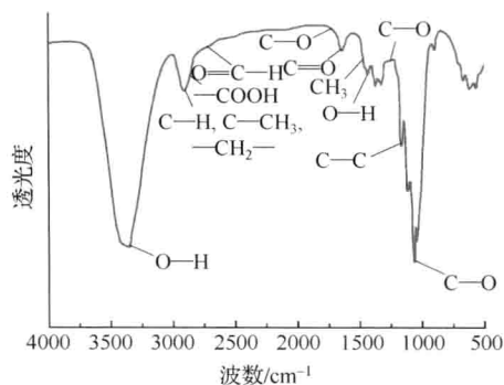
(c) 定性滤纸红外压片谱图
