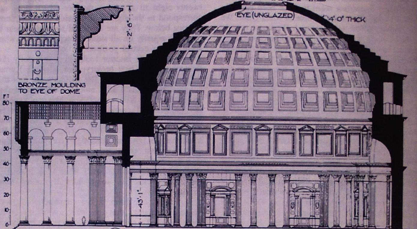
(A) SECTION THRO' PORTICO AND ROTUNDA
