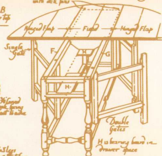
FRAMING DIAGRAM OF COMMON GATE LEG TAIL
