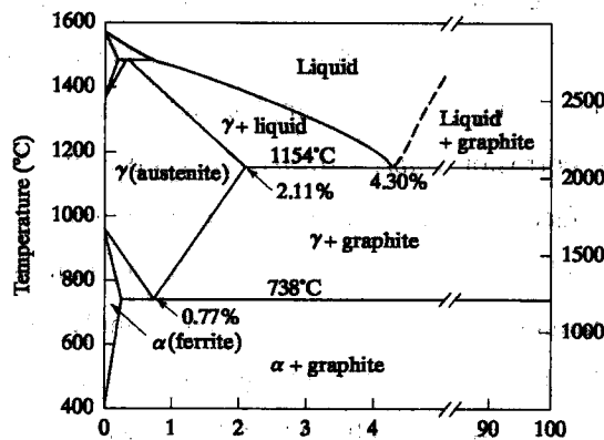
Fig.1.1 composition graphite(%)
