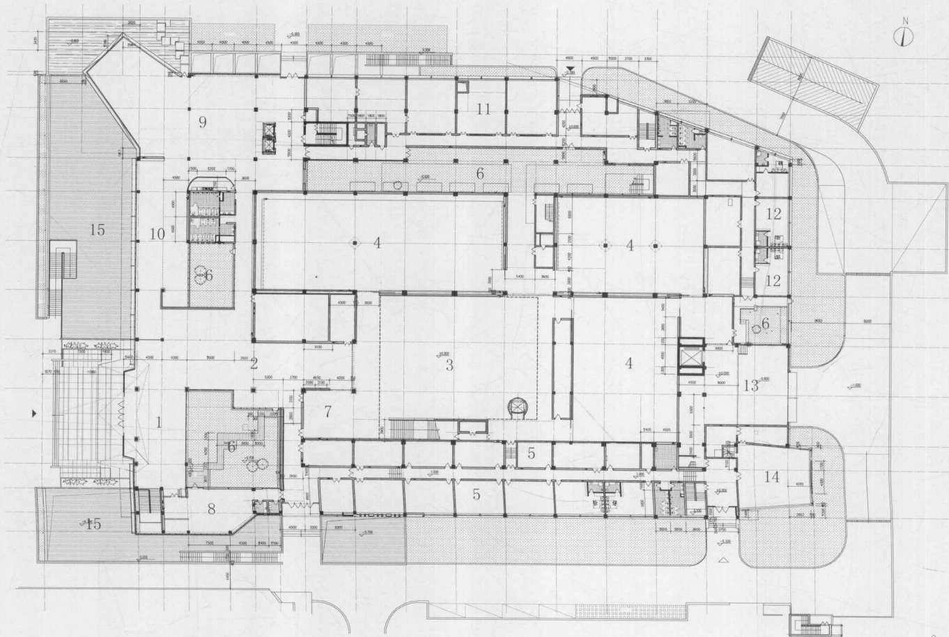
一层平面图 Ground Floor Plan
