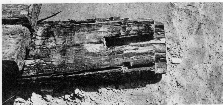
2. 垫木卯眼
