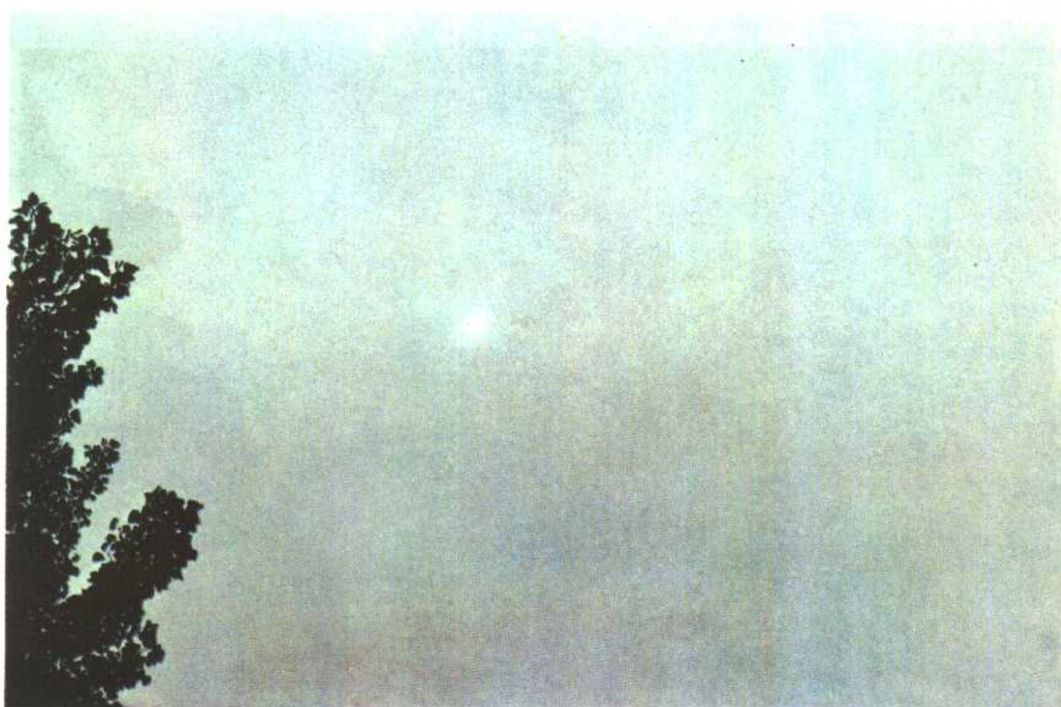
图2-31 透光高层云
