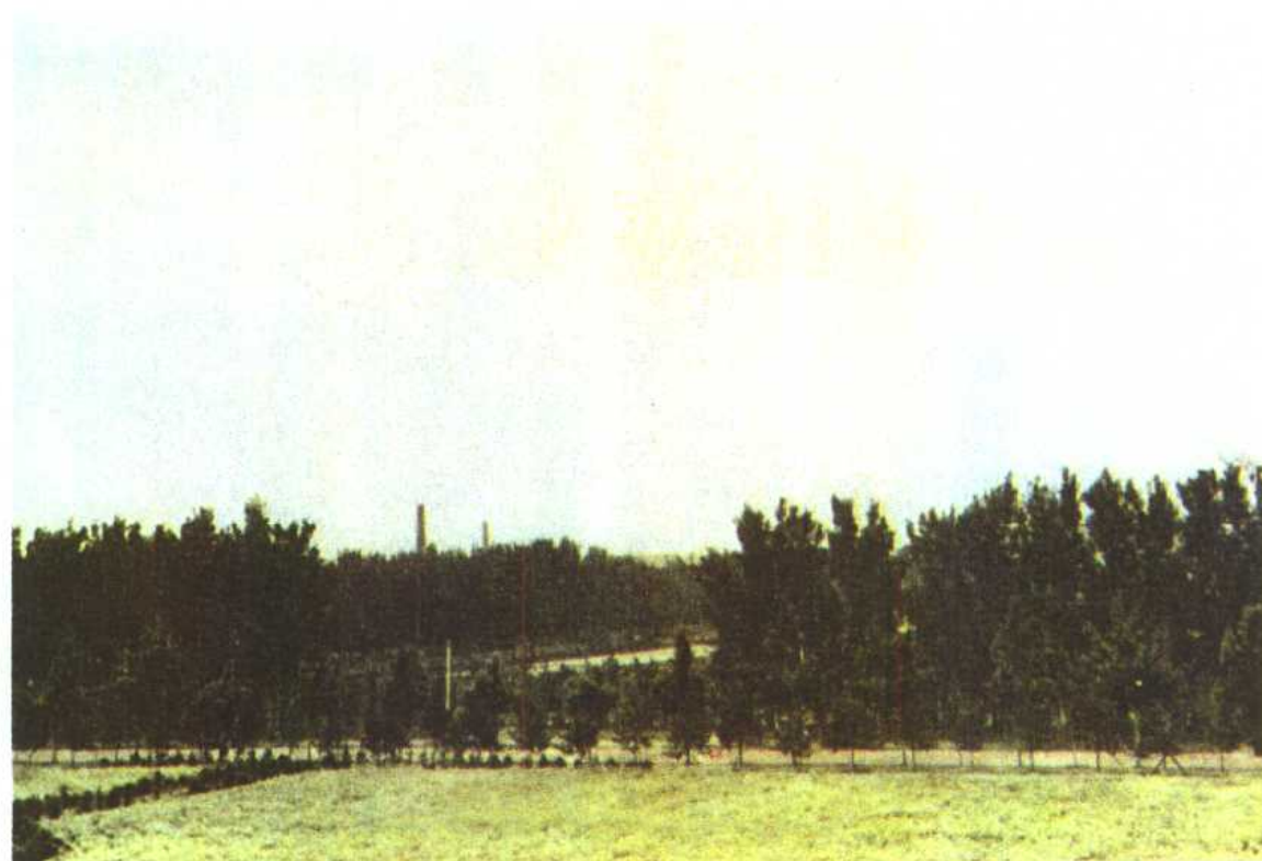
图2-32 蔽光高层云
