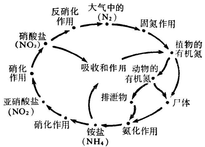
图绪-2 氮循环
