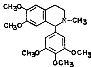
(15) \lambda_{281\text{nm}}
