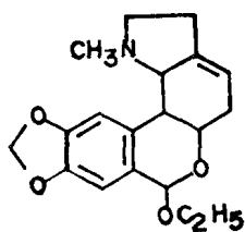
(28) \lambda_{239, 290\text{nm}}
