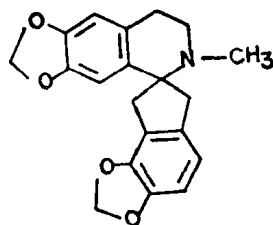
(27) \lambda_{240, 291\text{nm}}
