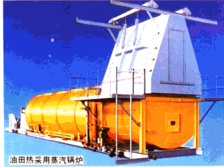
3-23t/h 油田热采用蒸汽锅炉 3-23t/h THERMAL RECOVERY STEAM GENERATOR FOR OIL FIELDS
