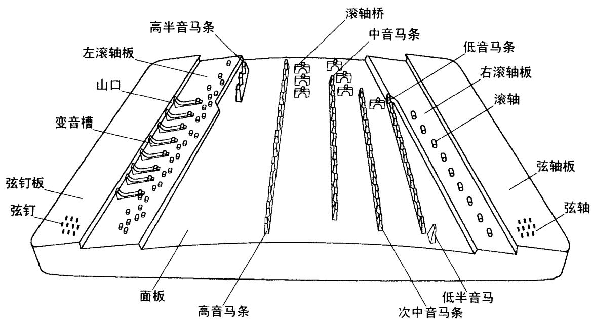
扬琴正面图
