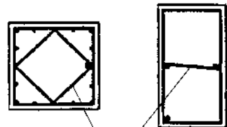
additional stirrup 附加箍筋
