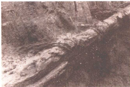
捍海塘护基木椿和横木捆绑情况
