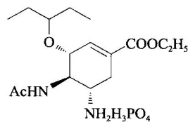
达菲 (Oseltamivir phosphate, Tamiflu)
