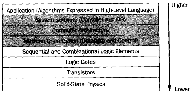
Figure P.1 Levels of abstraction in a computer system.
