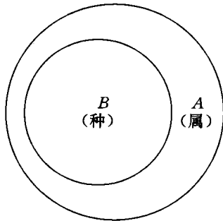
A \supset B
