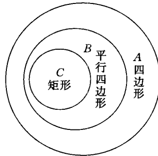
A \supset B \supset C
