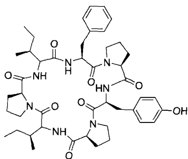
phakellistatin 1
