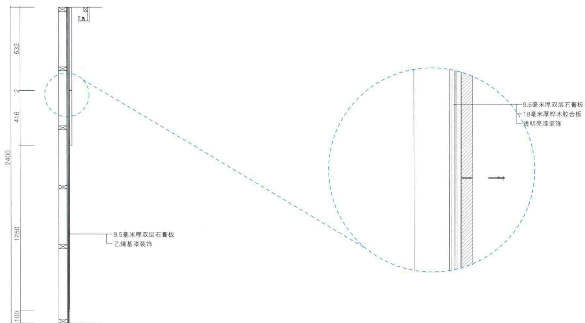
剖面图D
