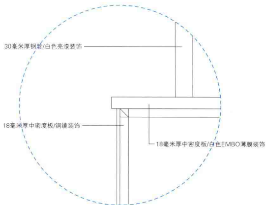
细节图B
