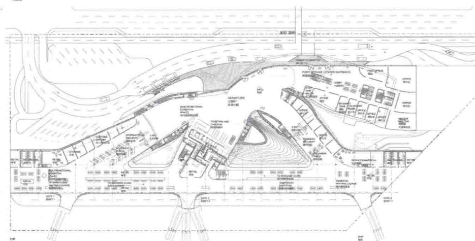
MAIN LEVEL PLAN - CRUISE DEPARTURES 主層-客輪出境 A. Top 1 level 1:500
