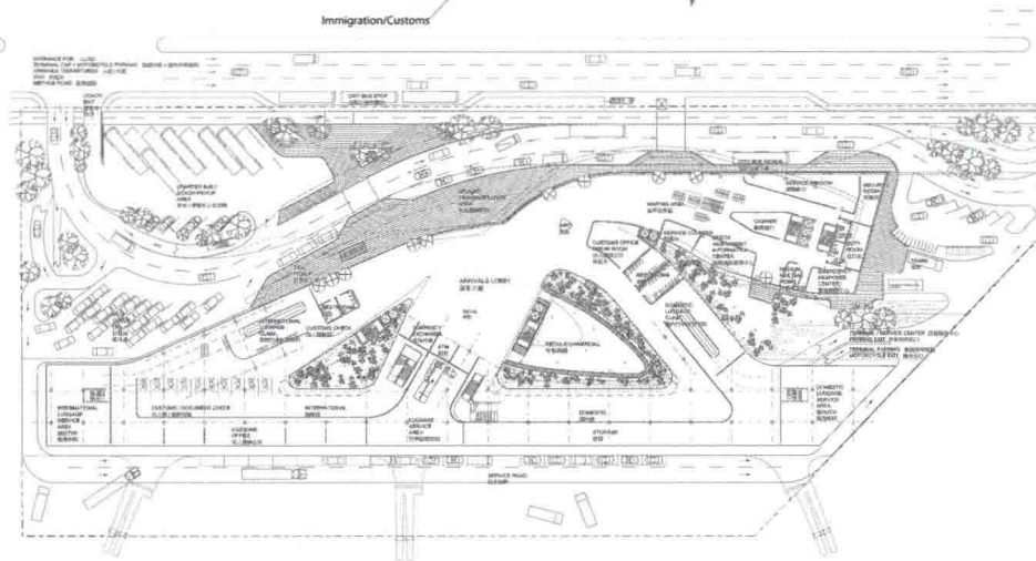
GROUND LEVEL PLAN - CRUISE ARRIVALS 港區層-客輪入境 On Level 1:500
