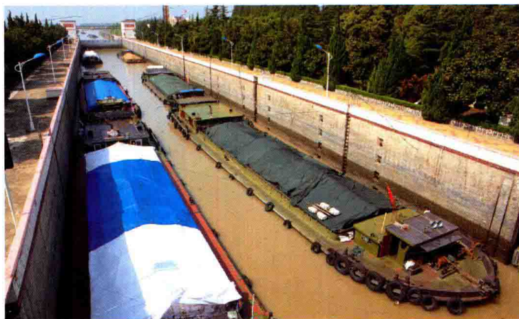
A ship lock on the China Grand Canal at Shaobo Town, Yangzhou, Jiangsu Province.
