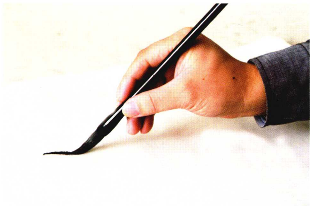
拖锋运笔
