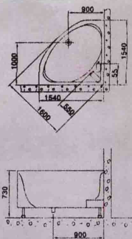
MODEL:AT-903 SIZE:1540X1540X730mm
