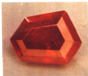
Cinnabar
